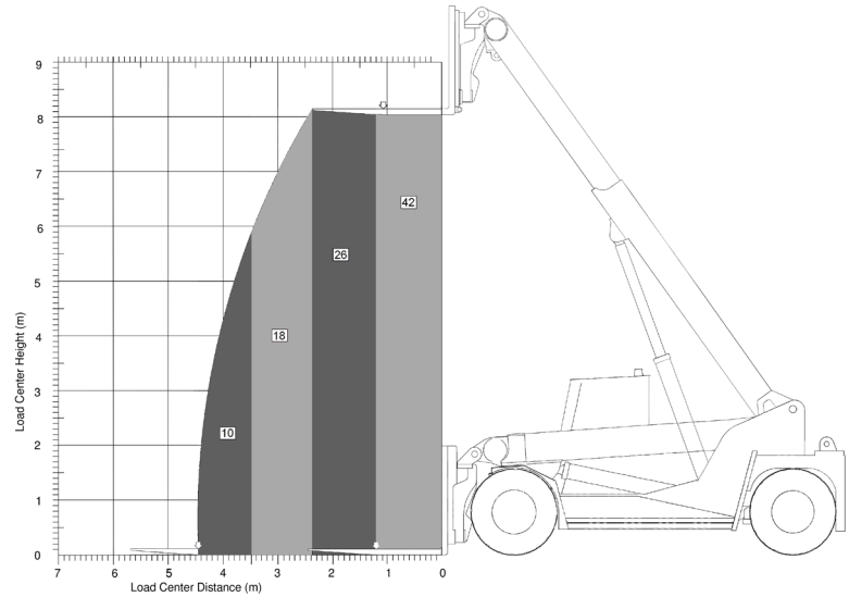
LIFTING CAPACITY DIAGRAM ML4212RC
